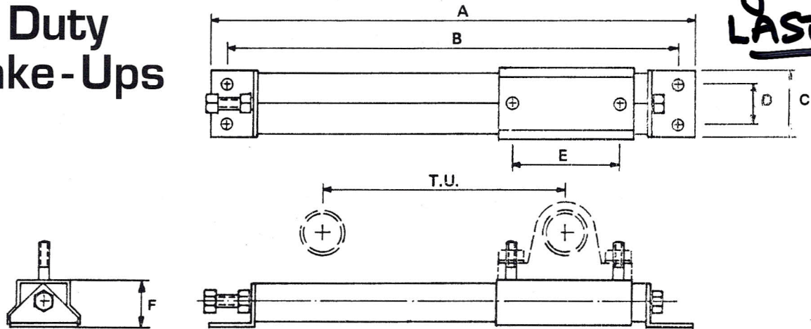
ABP Series Standard Duty Screw Take-Up
