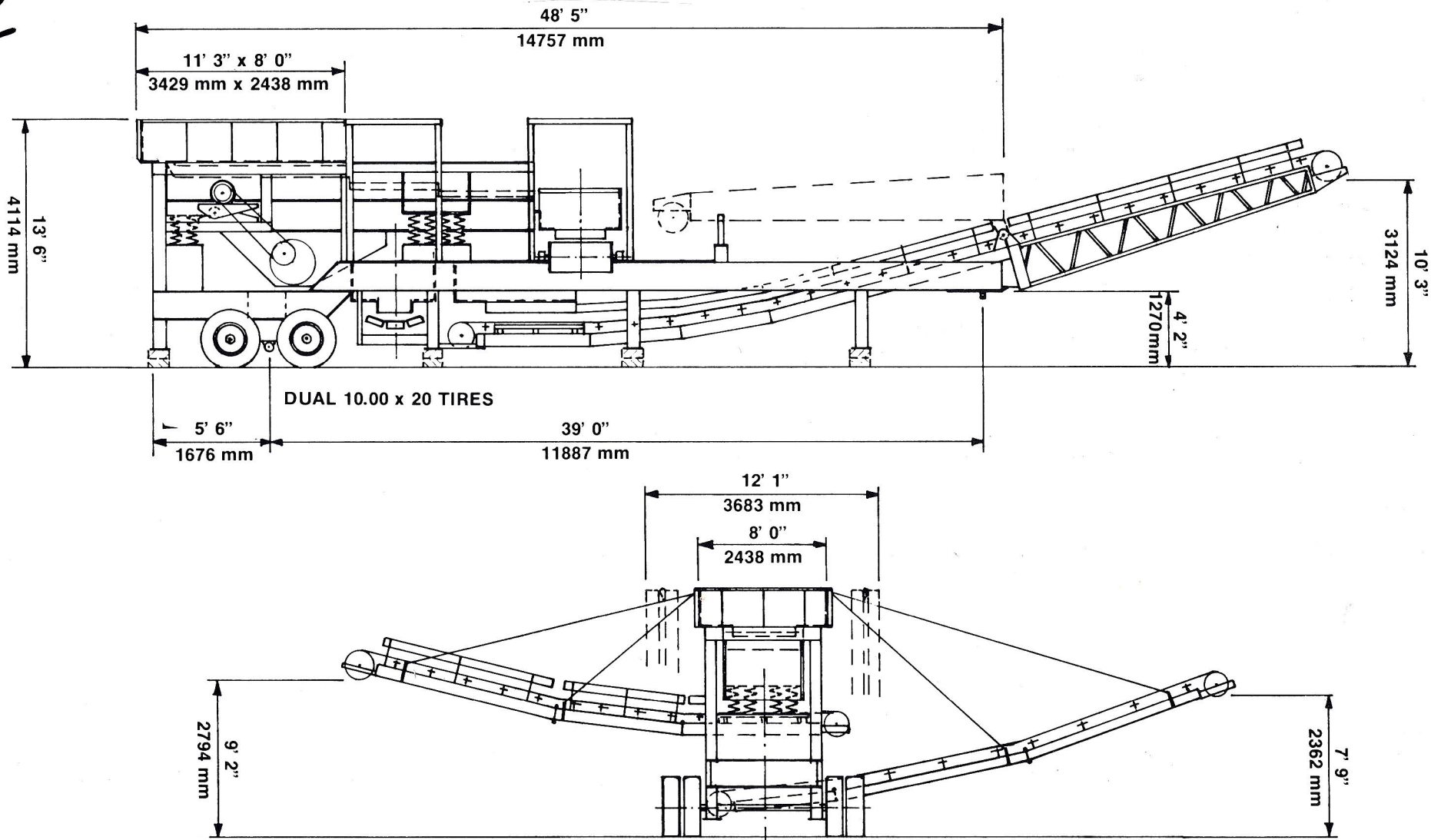
4' x 20' or 1219 x 6096 PORTABLE GRIZZLY FEEDER SORTING OF GABION STONE
